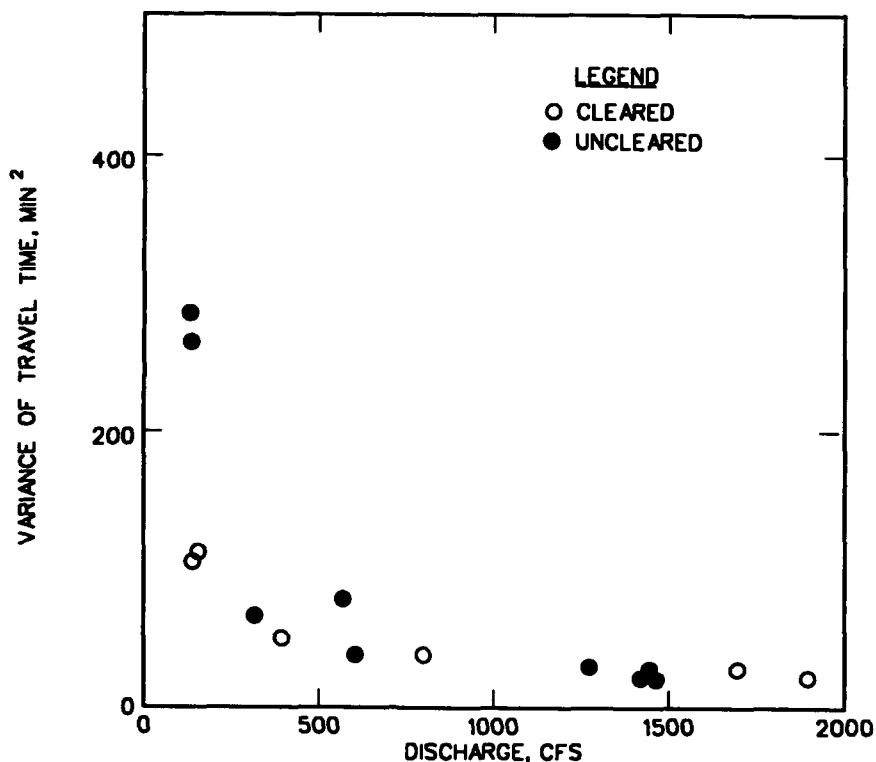
Figure 19. Dye test time-of-travel variance versus discharge
