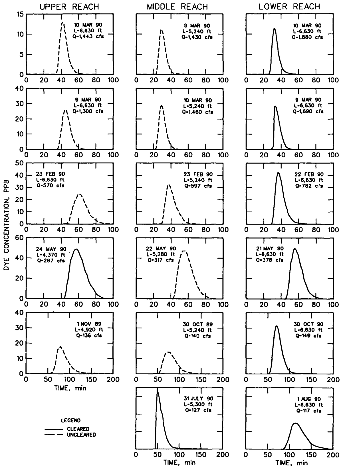
Figure 15. Dye curves
