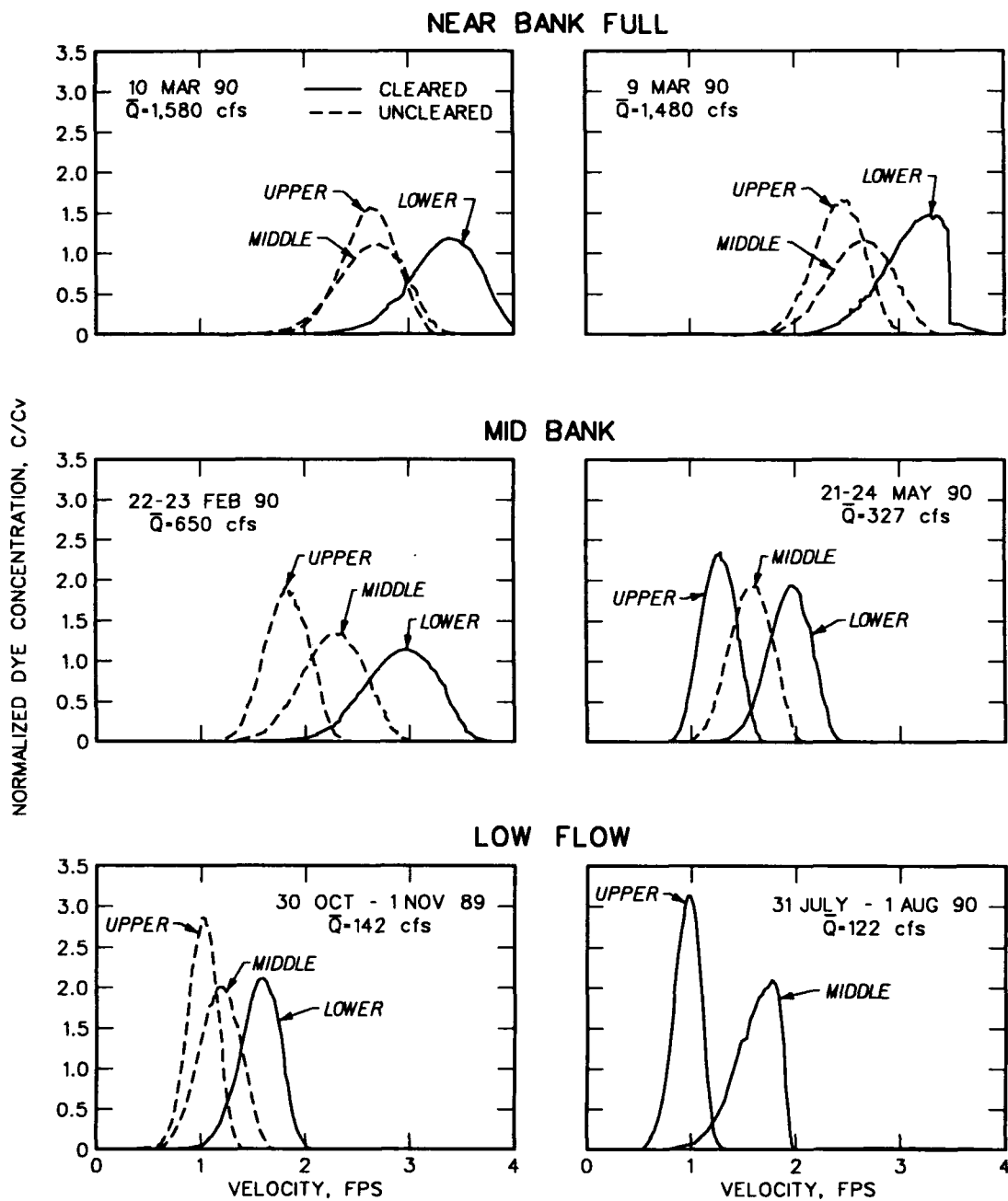
Figure 16. Normalized dye concentration versus reach mean velocity
